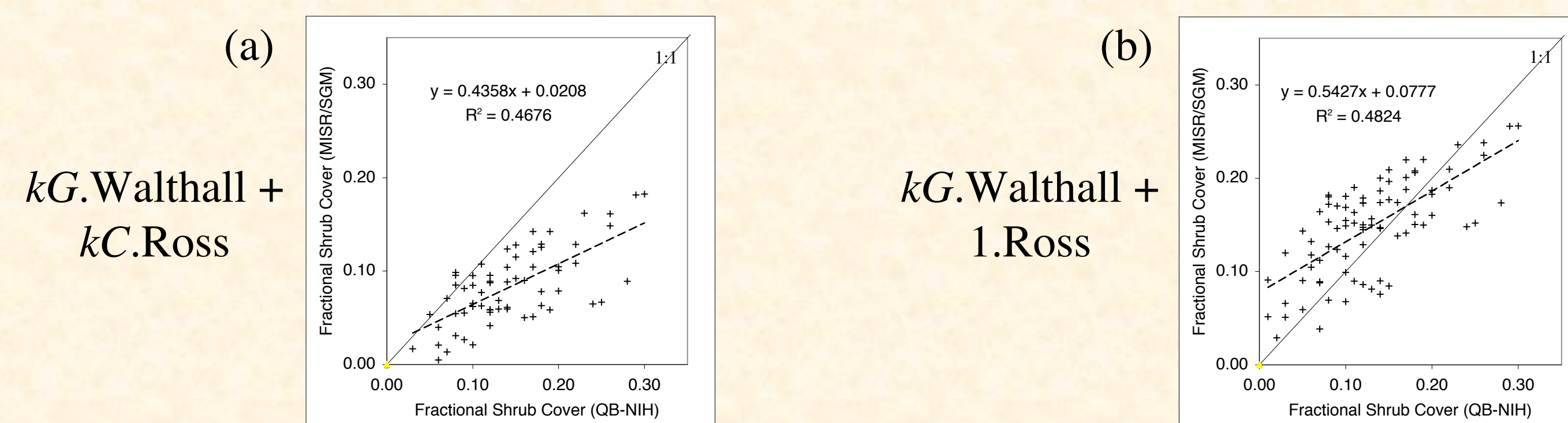
Figure 6. Scatter plots of retrieved vs measured shrub cover, (a) SGM (b) SGM with kC = 1
