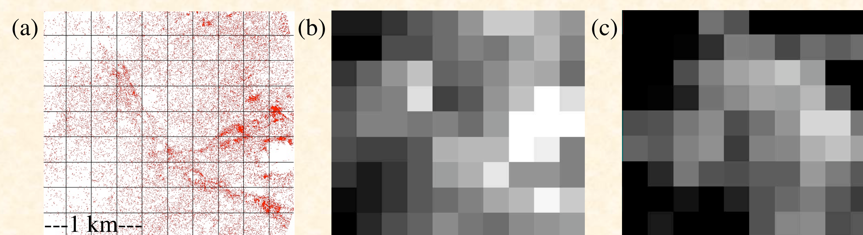
Figure 5. (a) QuickBird shrub map for pasture 12 in the Jornada, red=shrub, white=background (b) shrub cover aggregated to 250 m (c) retrieved using MISR via inversion of the SGM GO model.
