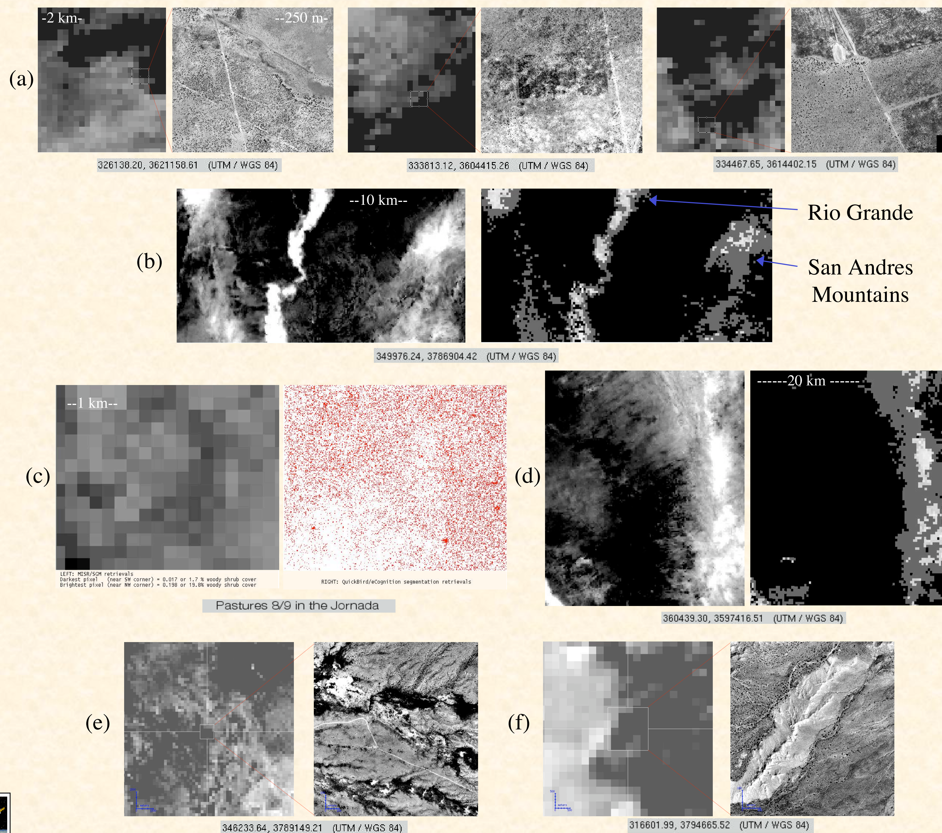
Figure 4. Retrieved woody plant cover maps (left side of each pair) vs: (a) IKONOS pan images (b) MODIS Vegetation Continuous Fields (VCF) % Tree Cover for the Sevilleta (c) QuickBird-derived shrub cover map for pastures 8/9 in the Jornada, red=shrub, white=background (d) MODIS VCF % Tree Cover for the Jornada (e) and (f) orthophotographs in the Sevilleta.
