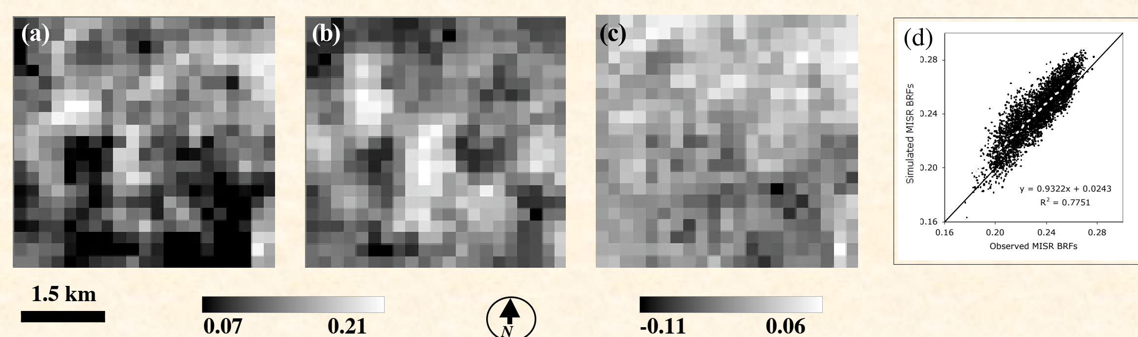
Figure 3. (a) Measured fractional woody cover from May 2001 IKONOS pan image (b) MISR/SGM fractional woody cover (black indicates failed inversions where cover is very low) (c) difference map (d) simulated MIRS red band BRFs in 9 looks vs. observed MISR data.
