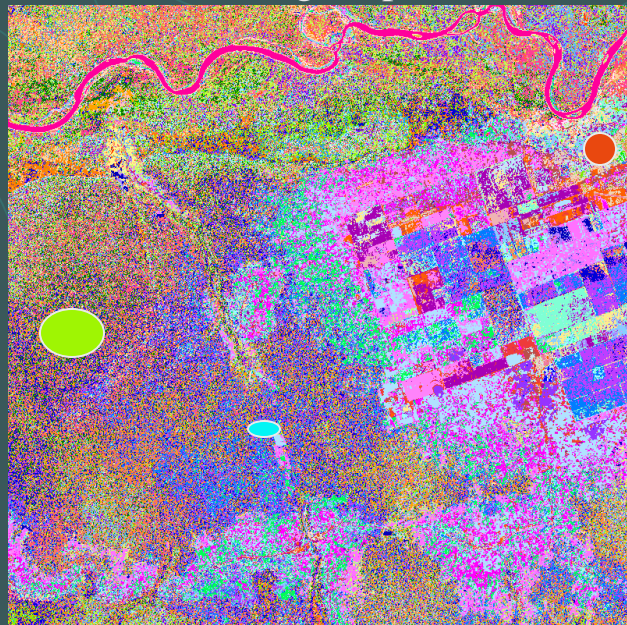
Clustering output
